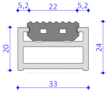
Detail with inlay rubber
